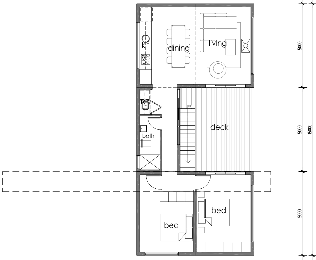
floor plan
