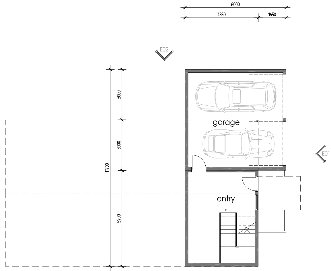
basement plan
