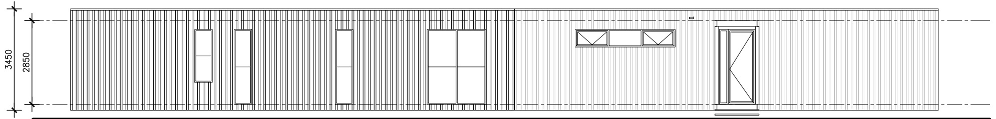
elevation 03
